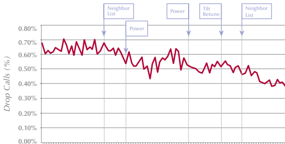
Drop Calls Improvement with Ultima Mentor™
